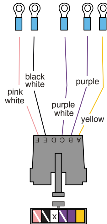
CONNECTOR C
