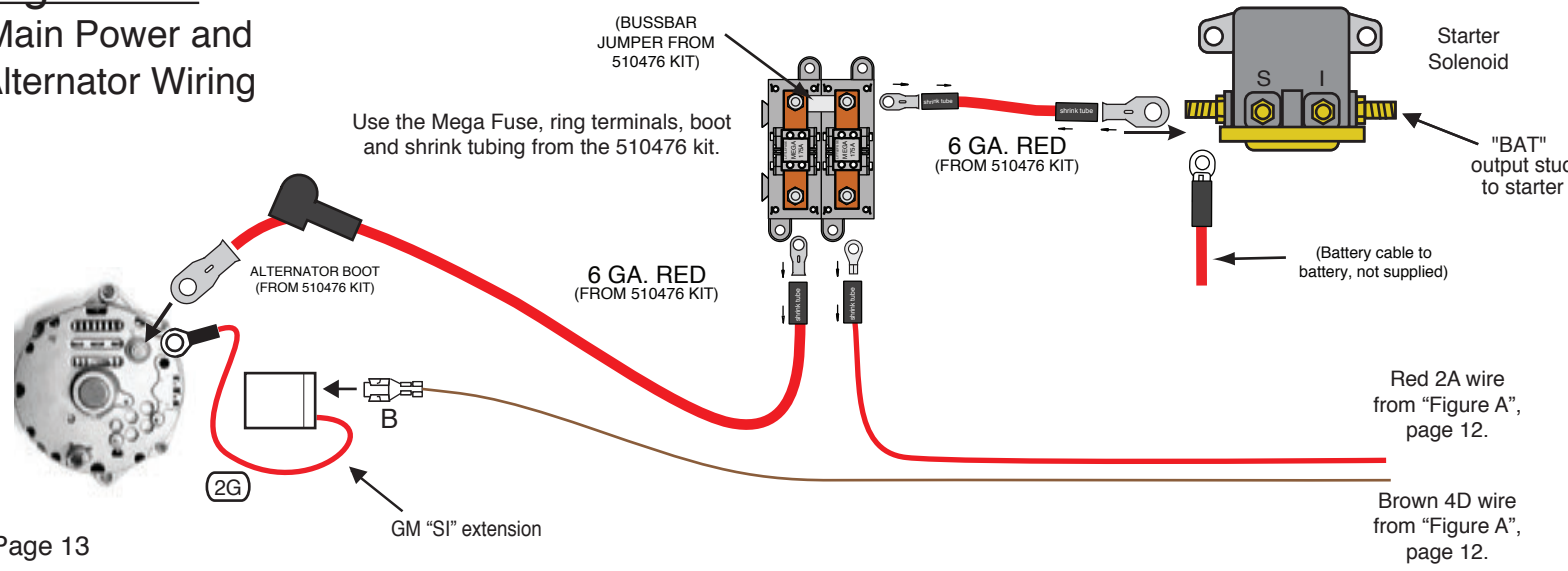
Figure "D" Shown is a typical NSS and Back Up Switch.
