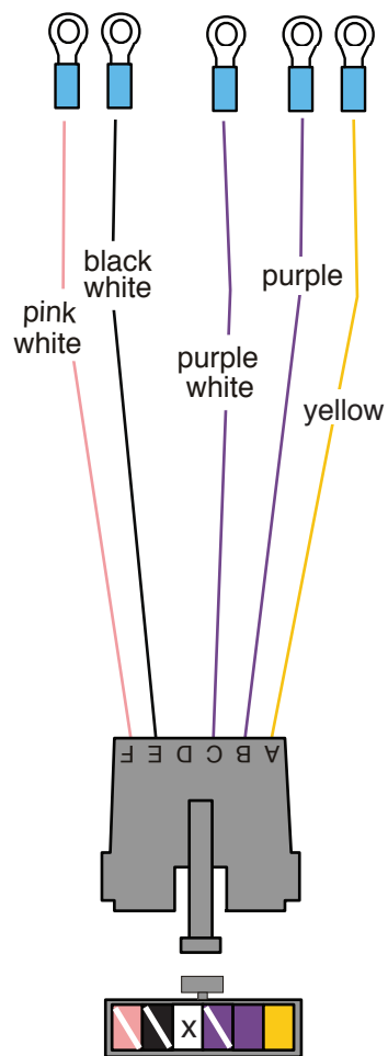
CONNECTOR C
