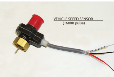
Typical 3 wire Autometer 5291 VSS connection
