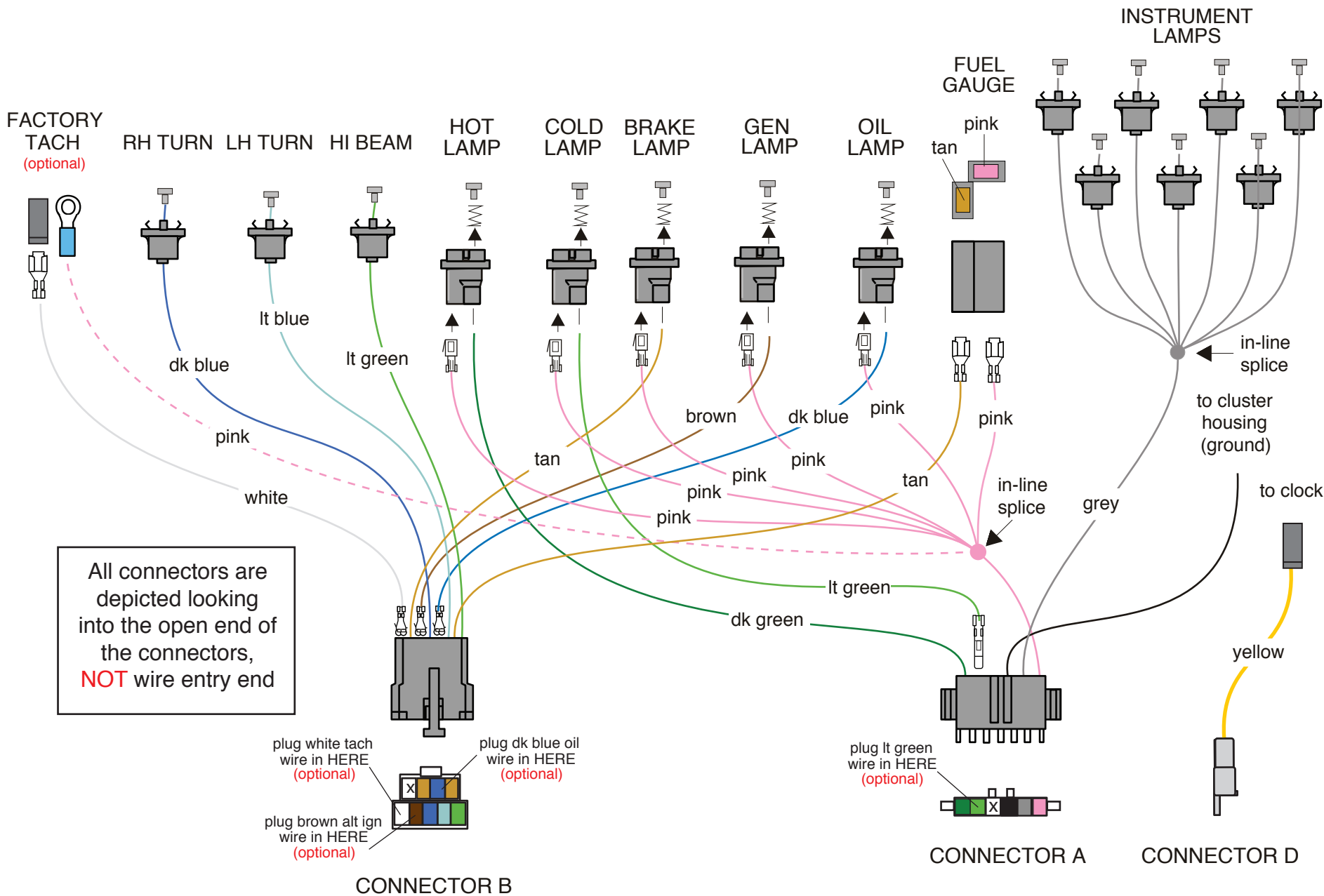
1965 CHEVY ALL FULLSIZE W/ WARNING LAMPS CLUSTER CONNECTIONS
