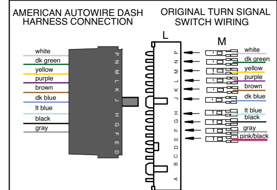
DIAGRAM 'B' - Stock 1965-68 Steering Columns Except 1965-66 With Tilt Column.
