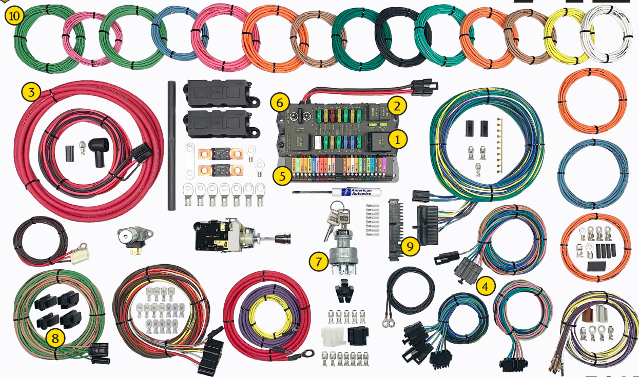
Fuse Panel Dimensions are 7.5" L x 4.5" W x 3.125" H
