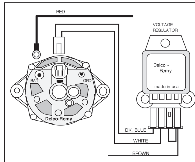
1963-1974 External Regulator
