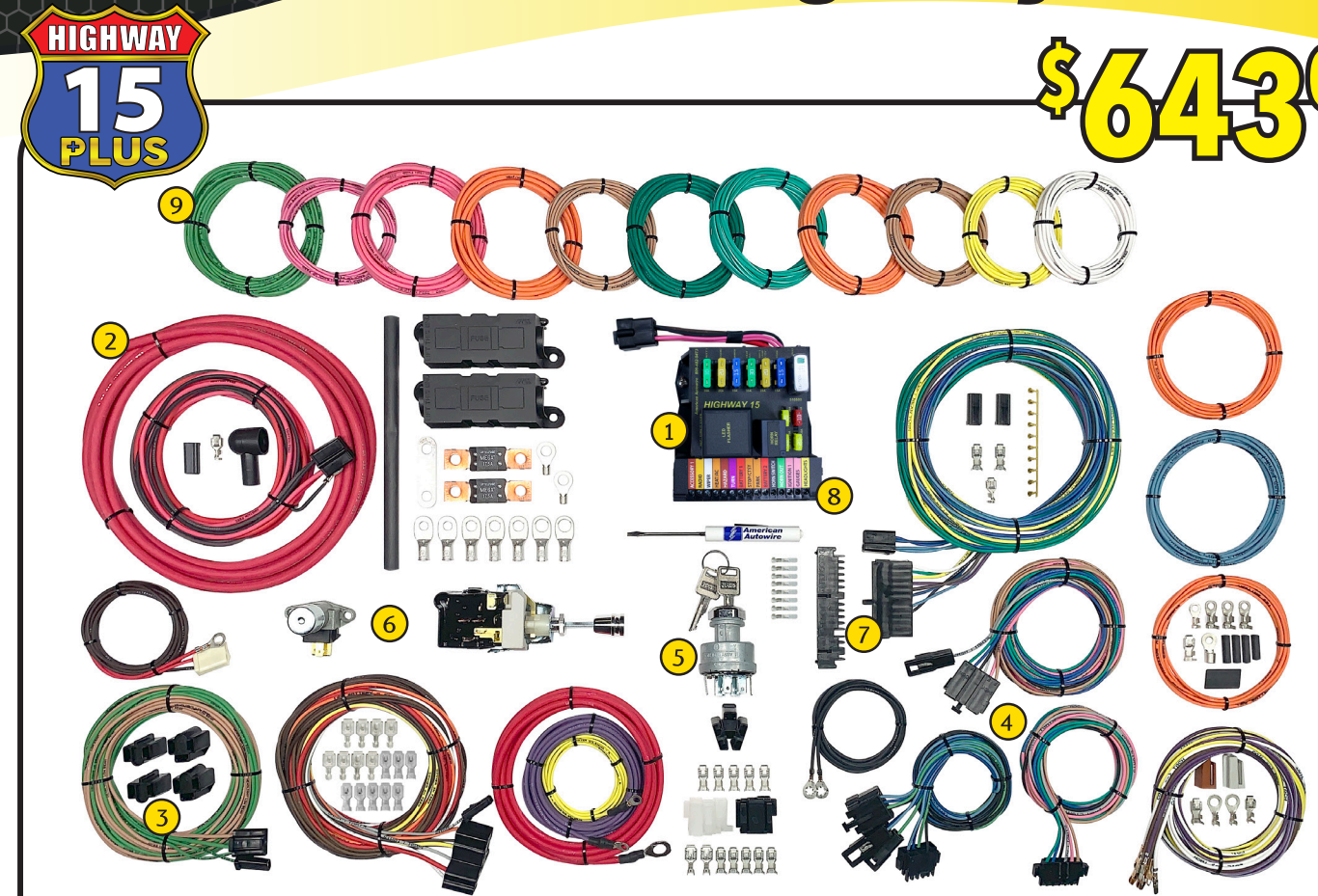
Fuse panel dimensions are 4.5" L x 4.5" W x 3.5" H
