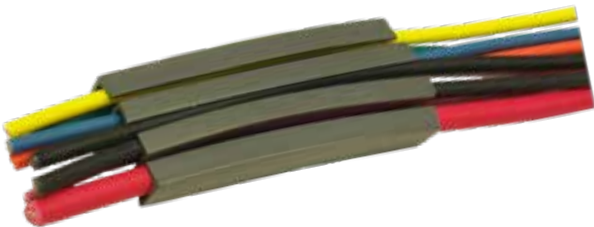
500716 Under-Carpet Protective Wiring Channel For use in under-carpet wire installation (8 ft section) 1" Wide x 3/8" Thick .....26.00 ea
