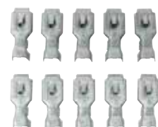
510286 Female 59 Series double .320 terminal 10 pcs ..... 6.00 ea
