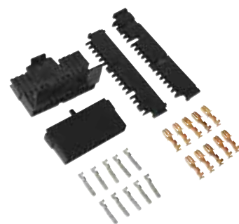
500428 GM Column Turn Signal Connector Set 3-7/8" & 4-1/4" Connector set allows the correct terminal and connector body connection to any 1969 or newer GM steering column without the use of exposed terminals or wiring. .... 12.00 set
