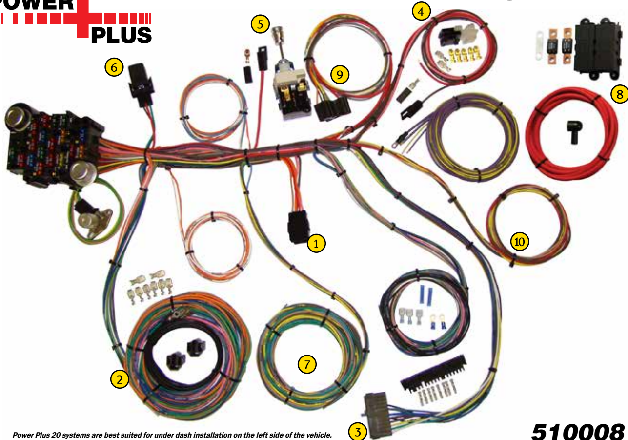
Power Plus 20 systems are best suited for under dash installation on the left side of the vehicle. Fuse panel dimensions are 5 1/2" L x 4 1/2" W x 3"H
