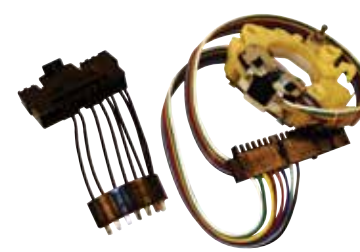
05698897 67-68 Camaro, 67-68 Chevelle, 67-68 Fullsize, 67-68 Nova, 1968 Cutlass, 67-68 Firebird, 68 GTO Turn Switch Assembly, all with column shift auto.trans, with & without tilt, "GUIDE-DELCO" type. NOTE: Emergency flasher actuator hole in outer collar has a "D" shape. ..... 50.00 ea
